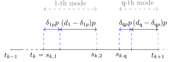
Fig. 3. Illustration of q modes with fast and slow dynamics.
