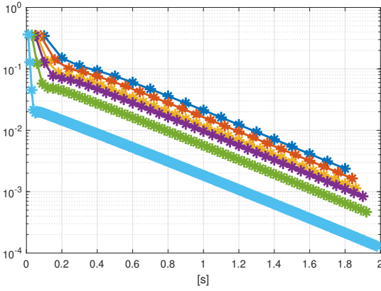
Fig. 9. Time evolution of the error \|m(t_k) - \mu(t_k)\| of Example 11 (the vertical axis is in logarithmic scale) for different values of the switching period: p = 0.1 s (blue line), p = 0.08 s (red line), p = 0.06 s (yellow line), p = 0.05 s (purple line), p = 0.03 s (green line) and p = 0.01 s (cyan line).
