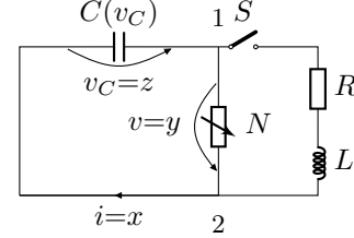
Fig. 2. A nonlinear switching electric circuit
