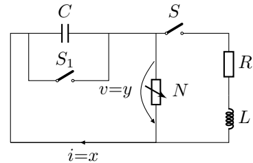
Fig. 4. The modified nonlinear switching electric circuit
