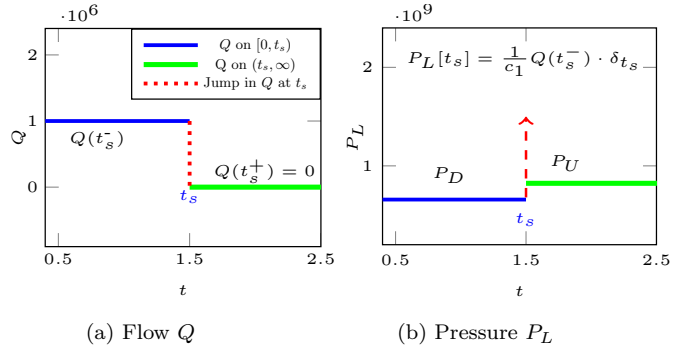
Fig. 2: Plot of solution x of Example (7) over time. In (a), red dotted line shows jump in Q and in (b) impulse in P_L due to presence of derivative of Q , moreover P_L[t_s] denotes impulse at t = t_s . The coefficient of \delta_{t_s} is the length of impulse.
